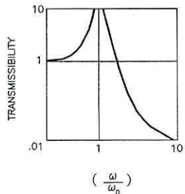
DISPLACEMENT RESPONSE – SINUSOIDAL FORCE NO DAMPING
